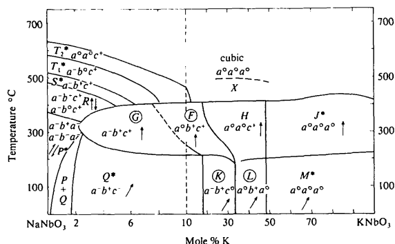
Fig. 1. Phase diagram of \text{Na}_{1-x}\text{K}_x\text{NbO}_3 . In each phase the tilt system is indicated according to the scheme of Glazer (1972). Vertical arrows indicate one-corner displacements and inclined arrows two-corner displacements of the cations. The phases with known structures are marked with asterisks. The circled letters show the phases studied in this work.
